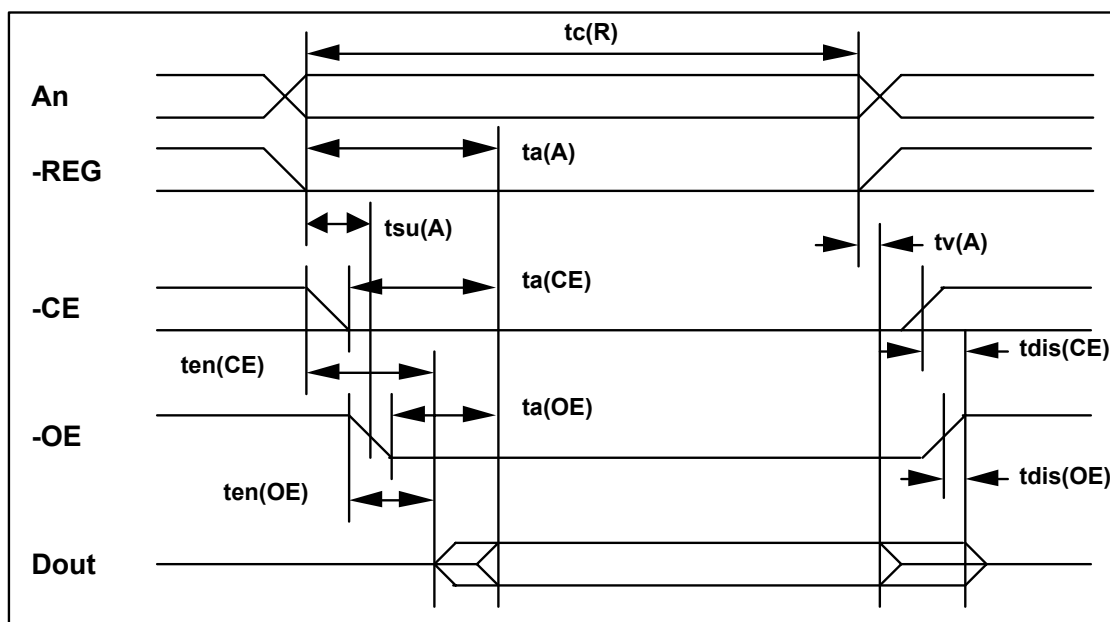
Figure 25: Attribute Memory Read Timing Diagram
