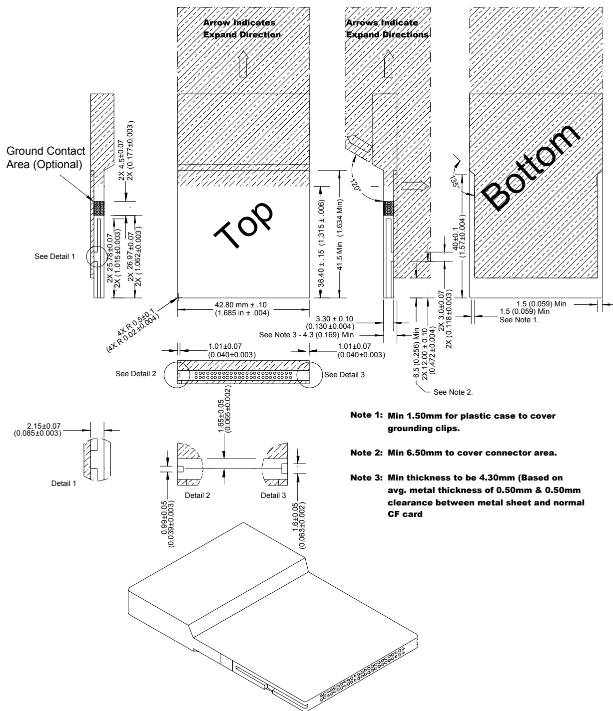
Figure 7: CF+ Extended Card Dimensions
