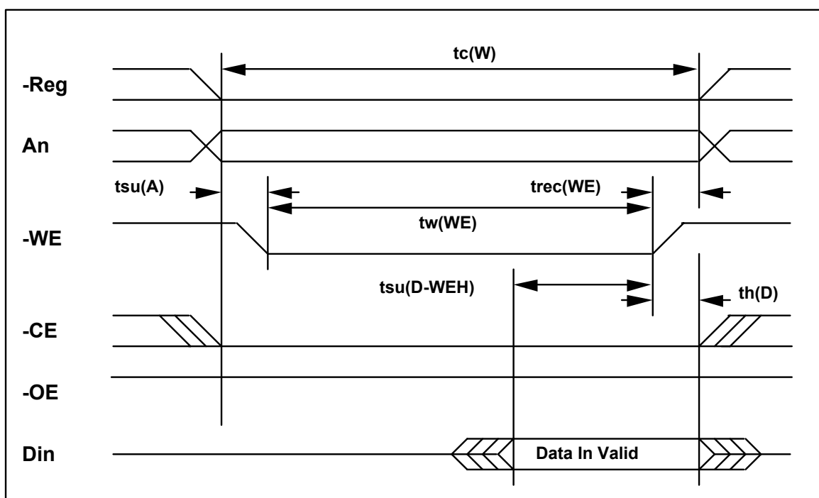
Figure 26: Configuration Register (Attribute Memory) Write Timing Diagram
