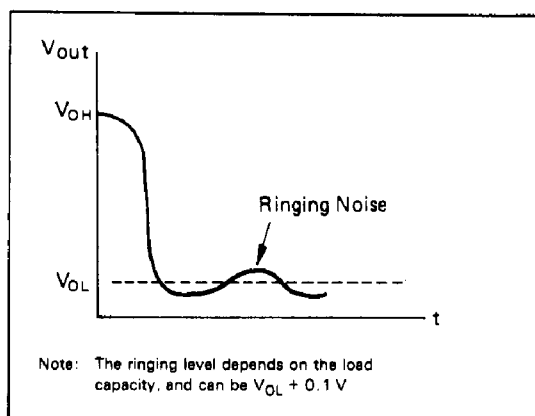
Figure 11. Ringing Noise
