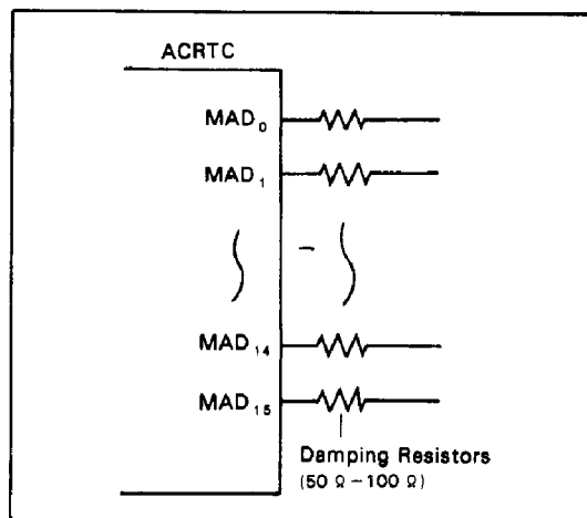
Figure 12. Damping Resistors
