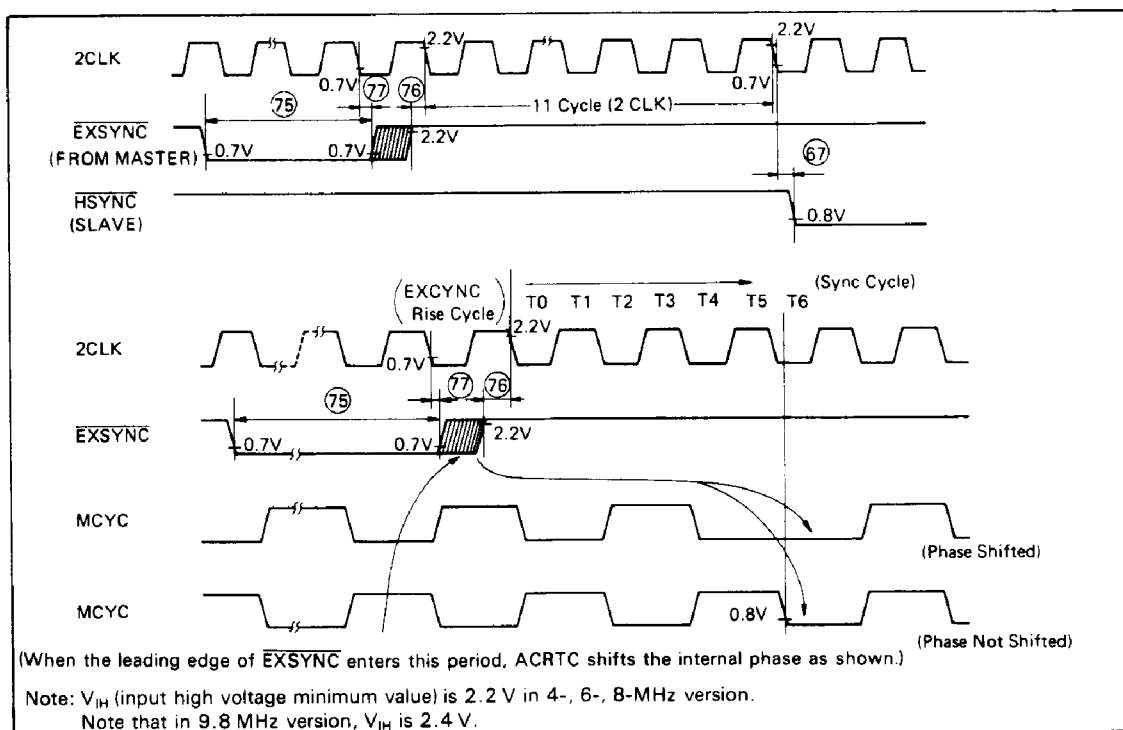
Figure 30. \overline{\text{EXSYNC}} Input Timing
