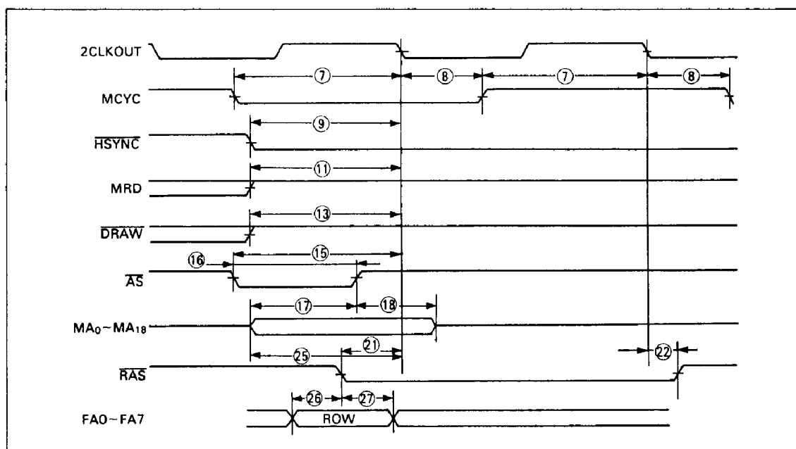
Figure 22. Refresh Cycle
